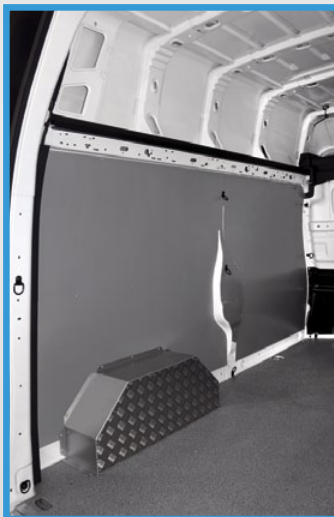
Vivaro/Trafic 2014/Talento 2016/NV300 H1: marble-look panel floor, side lining in painted metal sheet, wheel cover in aluminium/steel
