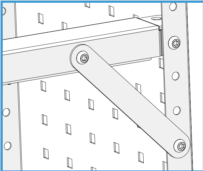
An ABC00002 bracket facing down.
