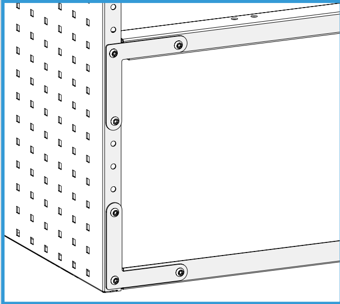
A pair of ABC00001 brackets providing upward and downward reinforcement.
