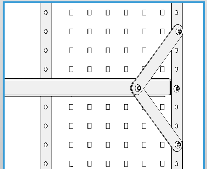
A pair of ABC00002 brackets mounted on the same angle part providing upward and downward reinforcement.
